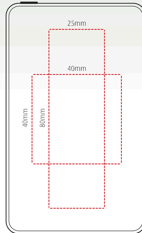
Laser engraving
